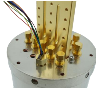
9-pin nanoD DC feed-thru (top view) Order # QMC-NANO9M-DCFT
