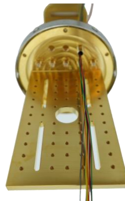
9-pin nanoD DC feed-thru (bottom view)
