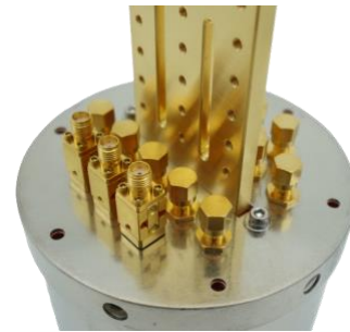
QMC-CRYOATTF-XXBLK Attenuator feed-thru Order # QMC-CRYOATTF-XXBLK
