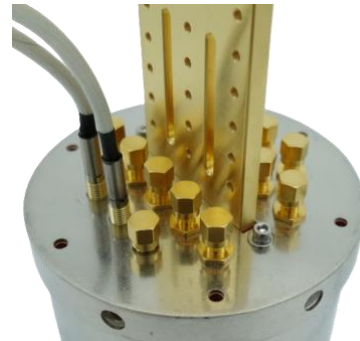
4-pin DC feed-thru (top view) Order # QMC-CAB-LEMO
