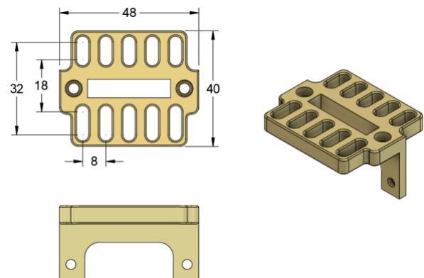
QMC-CRYOBRD Small mounting bracket for smaller Bluefors SD series dilution fridge
