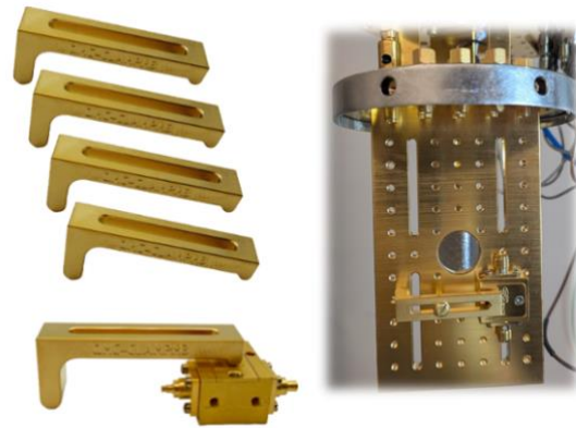
QMC-CRYOBRD Mounting Clamps Order # QMC-CLAMPM3
