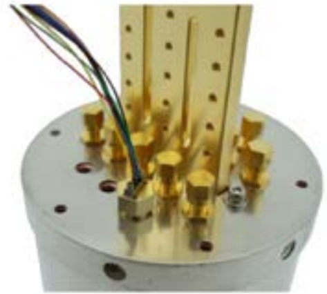
9-pin Omnetics nanoD DC feed-thru (top view)
