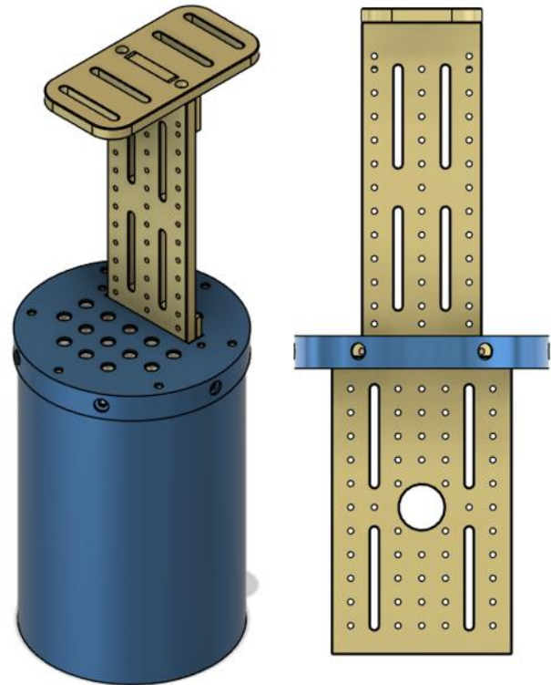
QMC-CRYOBRD-04SiC-offset
