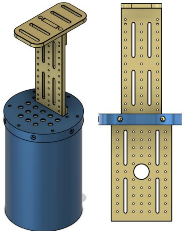
QMC-CRYOBRD-03SiC-offset
