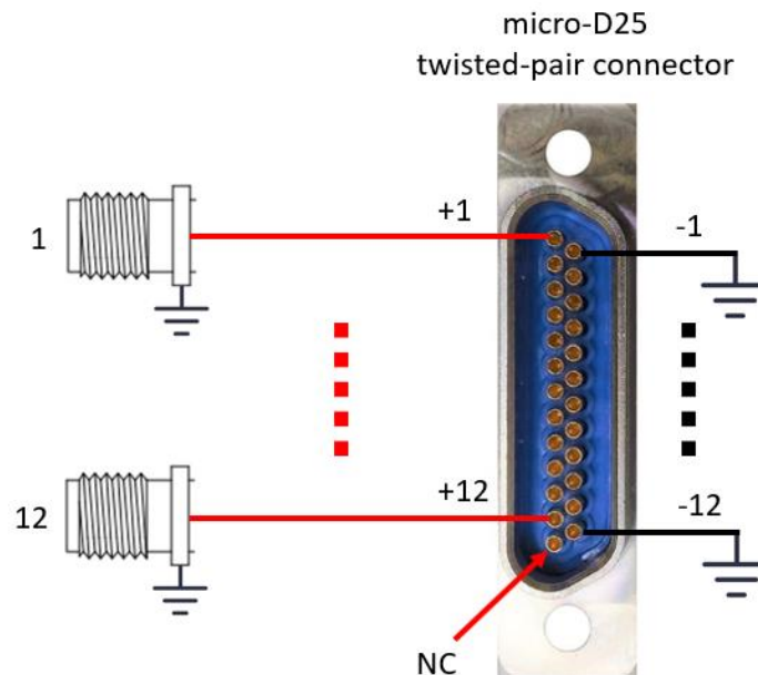
Figure 1. Wiring diagram
